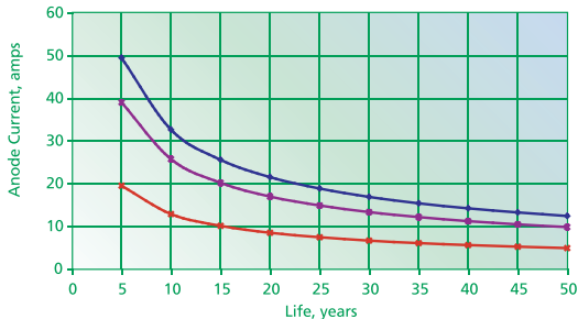
LIDA® Tubular Anode Life in Mud
